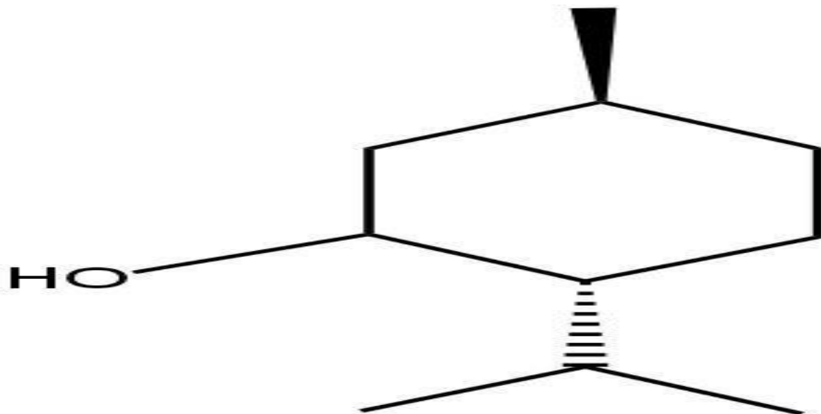
menthol's structure
